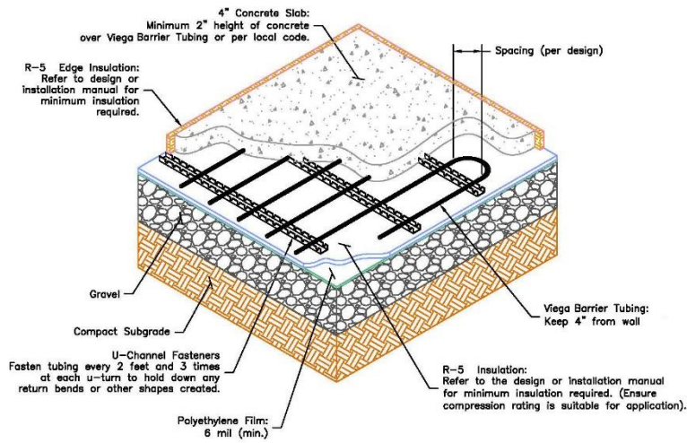
Figure 7 In-Slab – U-Channel
