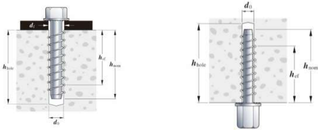
FIGURE 1—CELO BTS HEX WASHER HEAD DETAIL (Left Picture) AND CELO BTS HEX COUPLER HEAD INTERNALLY THREADED ANCHOR DETAIL (Right Picture)
