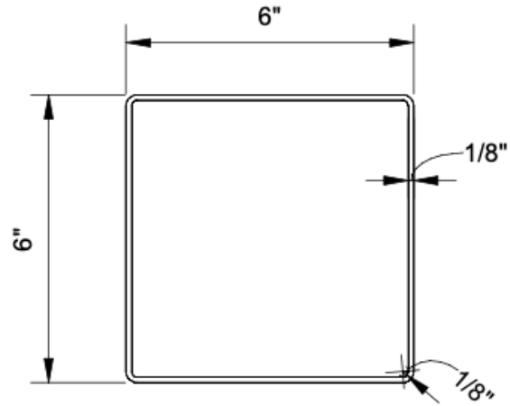
FIGURE 3—NEW CASTLE SUPPORT POST
