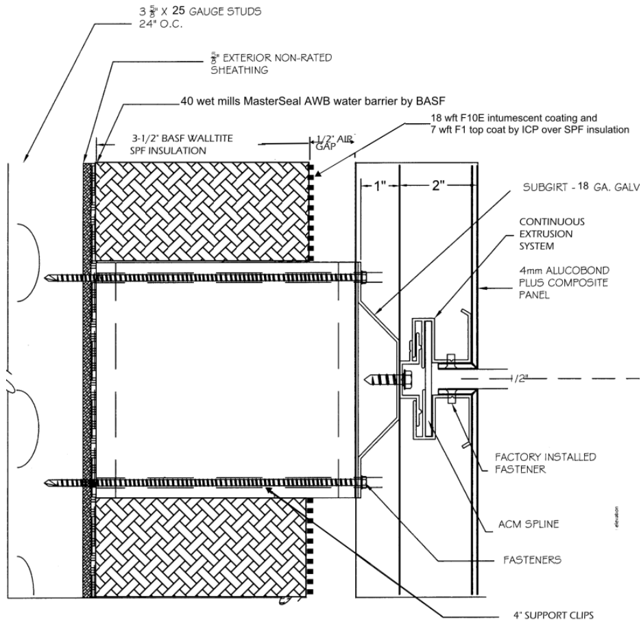
FIGURE 2—HORIZONTAL JOINT 1
