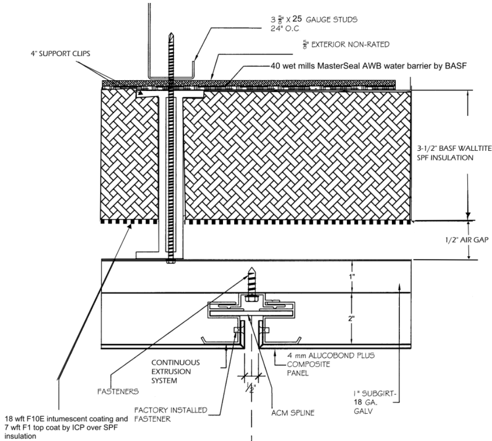
FIGURE 1—VERTICAL JOINT 1
