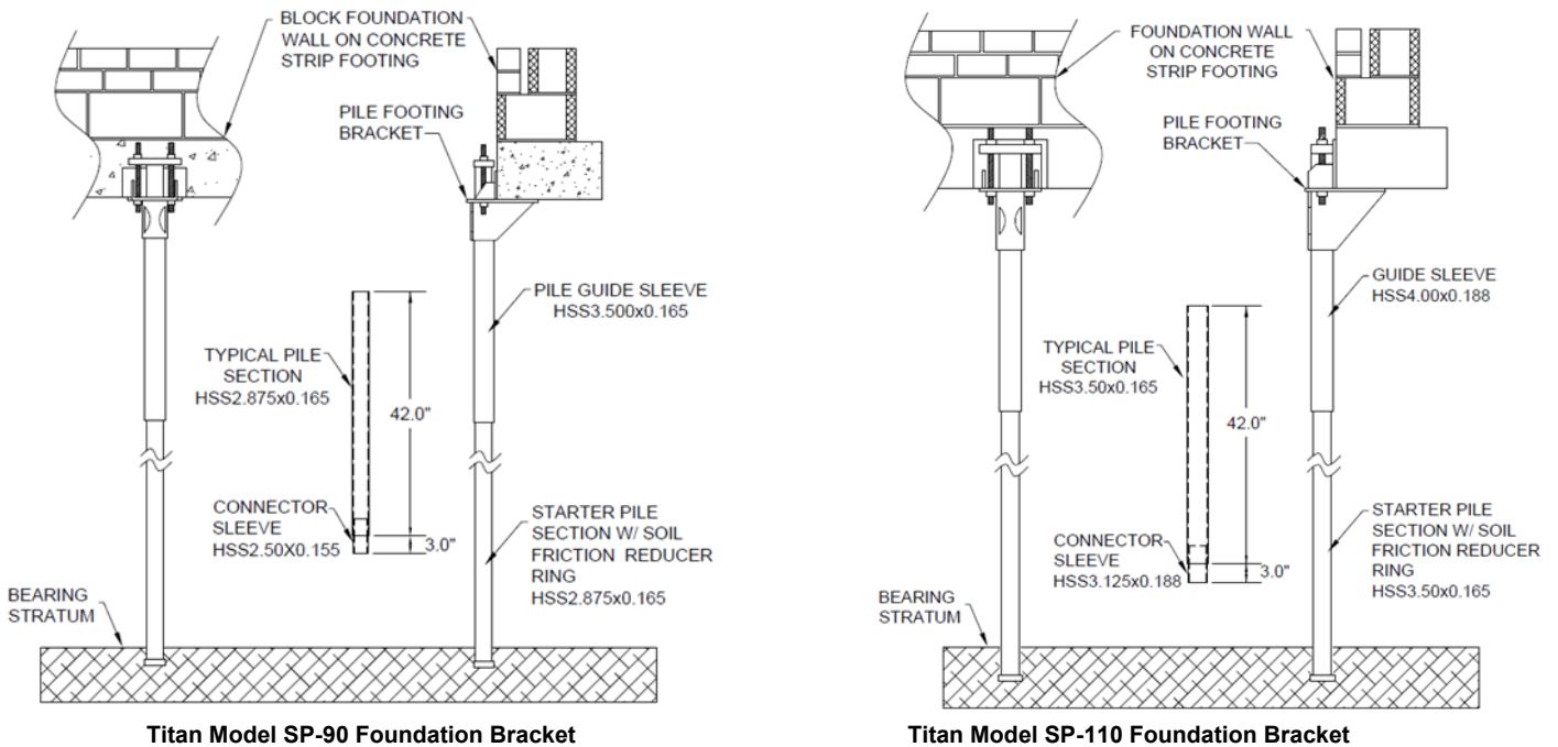
FIGURE 1 – TITAN FOUNDATION BRACKETS
