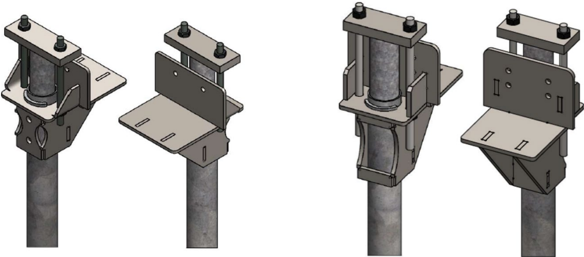
SP-110 Bracket Assembly
