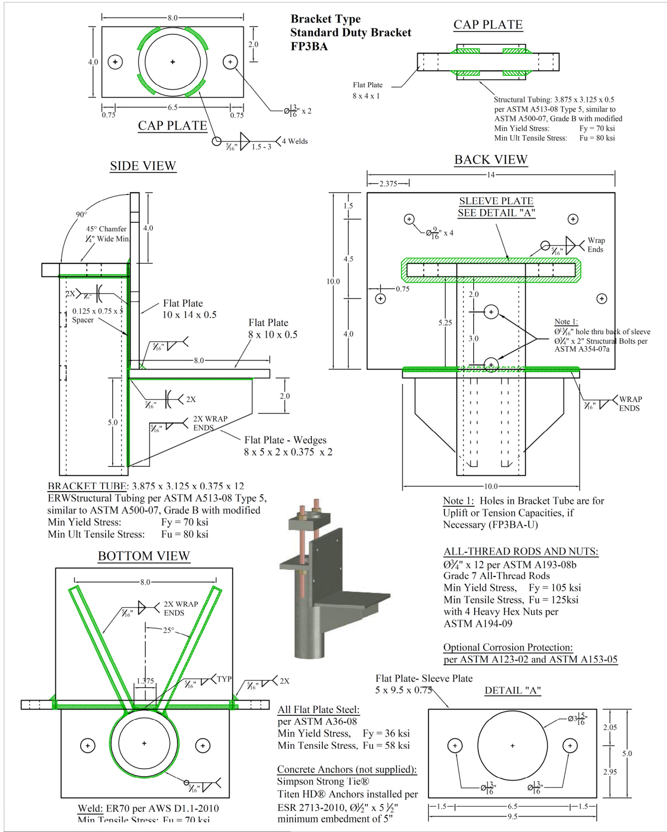
FIGURE 1—GRIP TITE® PUSH PIER SYSTEM BRACKET ASSEMBLY
