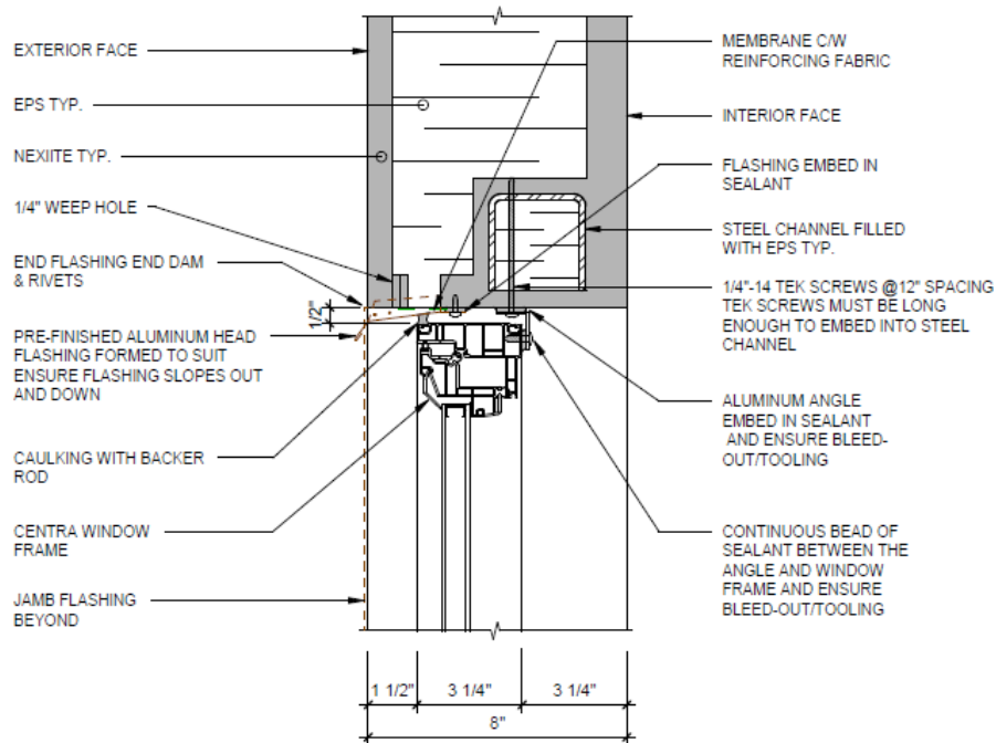
FIGURE 6—TYPICAL WINDOW HEAD DETAIL
