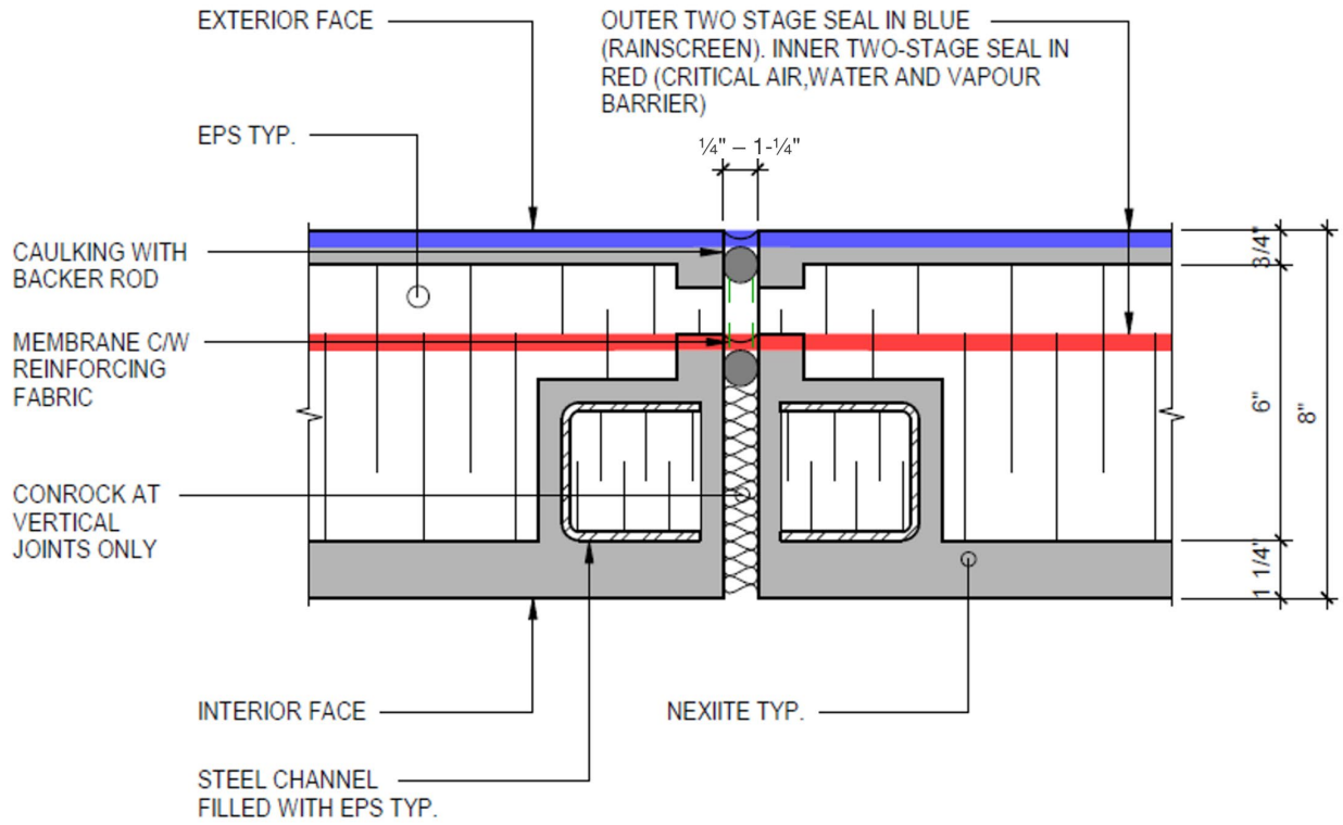
FIGURE 2—TYPICAL VERTICAL PANEL JOINT DETAIL
