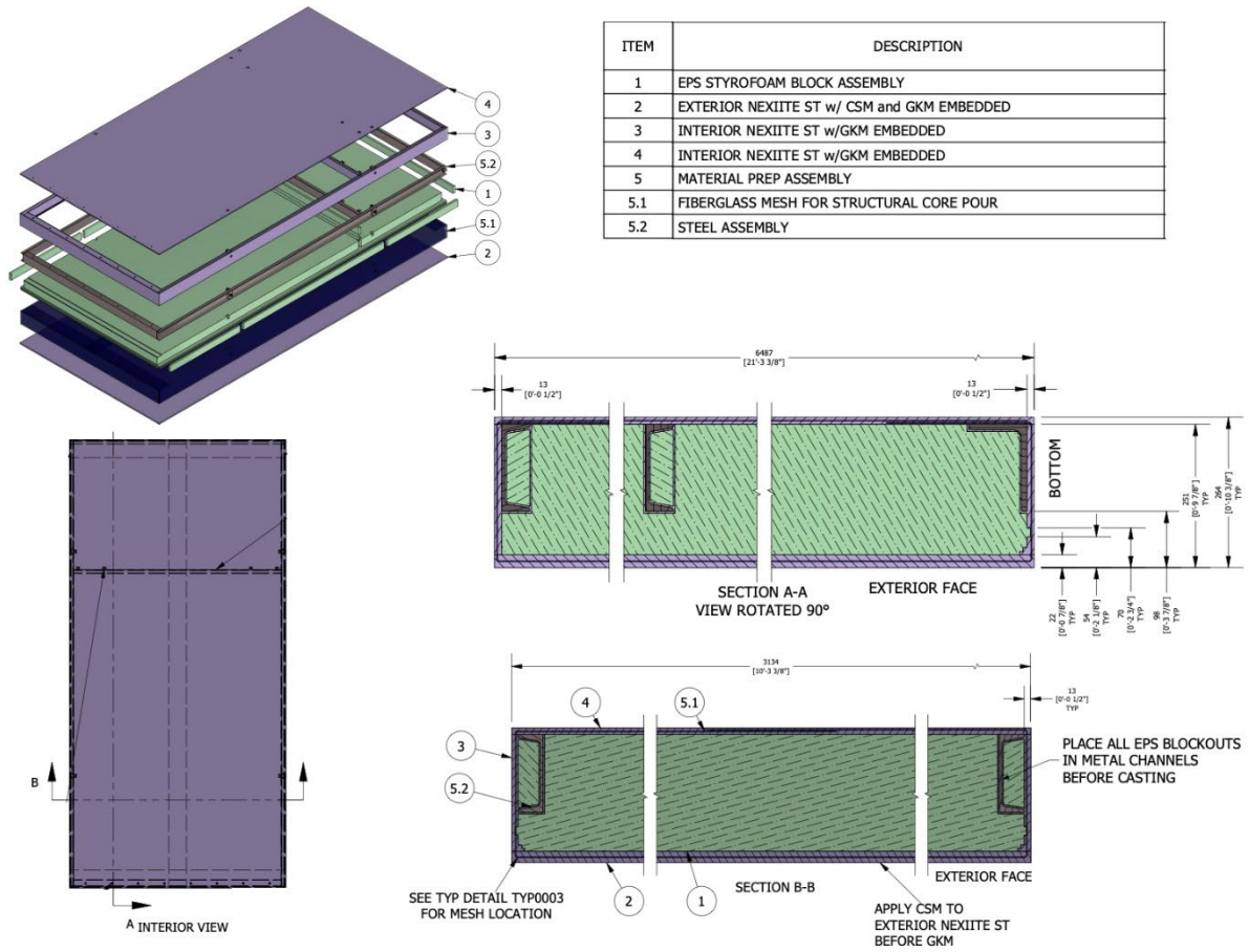
FIGURE 1—TYPICAL NEXII HPE PANEL
