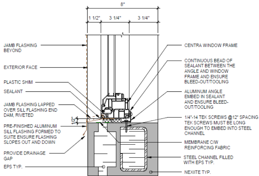
FIGURE 7—TYPICAL WINDOW SILL DETAIL
