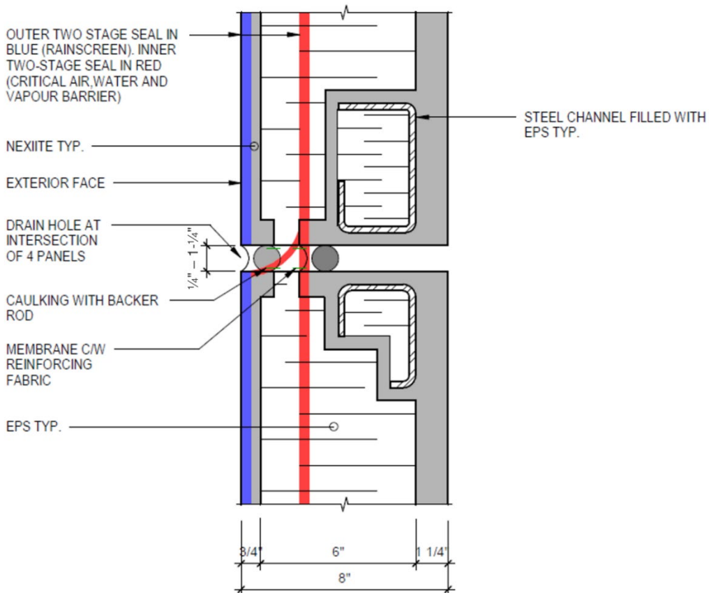
FIGURE 3—TYPICAL HORIZONTAL JOINT DETAIL
