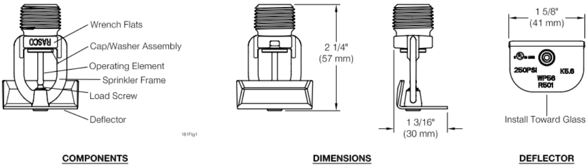
FIGURE 1—PENDANT VERTICAL SIDEWALL SPRINKLER
