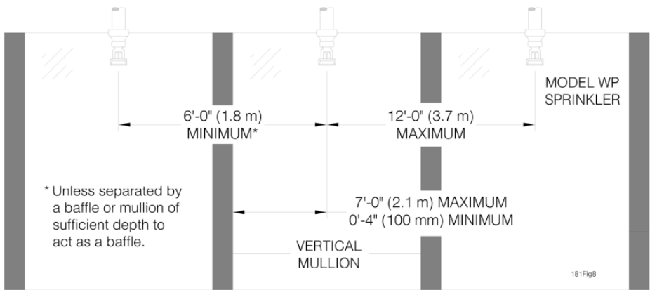
FIGURE 4—PENDANT VERTICAL SIDEWALL SPRINKLER SPACING
