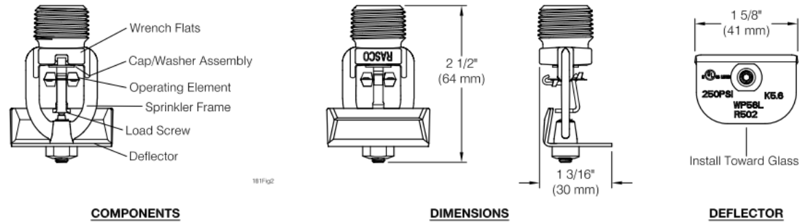
FIGURE 2—PENDANT VERTICAL SIDEWALL SPRINKLER
