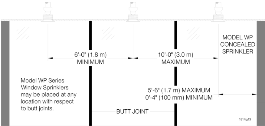
FIGURE 5— CONCEALED PENDANT VERTICAL SIDEWALL SPRINKLER SPACING
