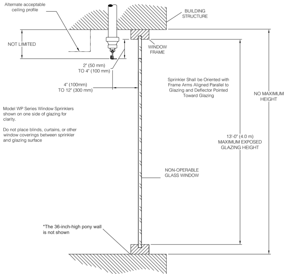
FIGURE 6—PENDANT VERTICAL SIDEWALL SPRINKLER INSTALLATION
