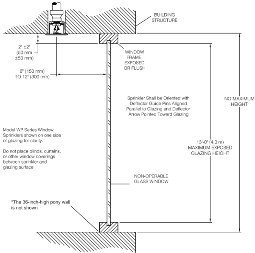
FIGURE 7—CONCEALED PENDANT VERTICAL SIDEWALL SPRINKLER INSTALLATION
