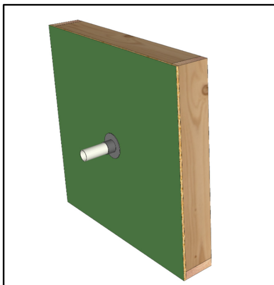
FIGURE 1 – TYPICAL FLASHING FOR THROUGH WALL PENETRATION
