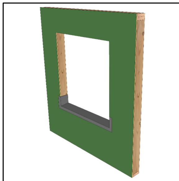
FIGURE 2 – TYPICAL FLASHING FOR WINDOWSILL PAN
