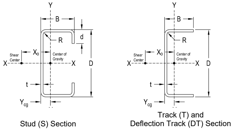
FIGURE 1—STUD AND TRACK GEOMETRY
