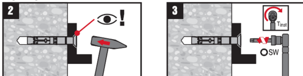
FIGURE 5—MANUFACTURER'S PRINTED INSTALLATION INSTRUCTIONS (continued)
