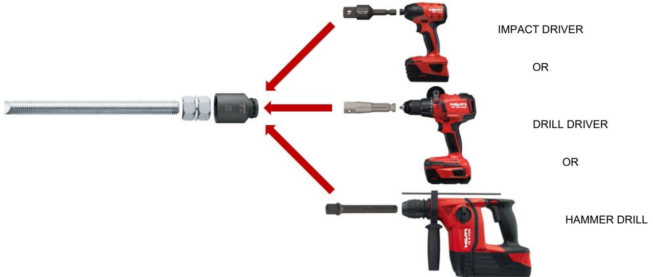
THREADED ROD WITH SETTING TIP, DOUBLE NUT, SOCKET, DRILL ADAPTERS, AND SETTING DRILLS
