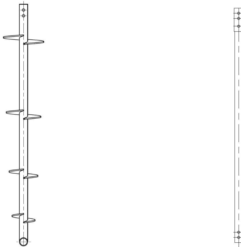
FIGURE 1—TYPICAL HELICAL PILE LEAD AND EXTENSION WITH COUPLER
