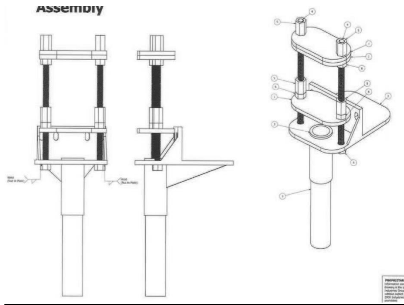
FIGURE 2—REPAIR BRACKET
