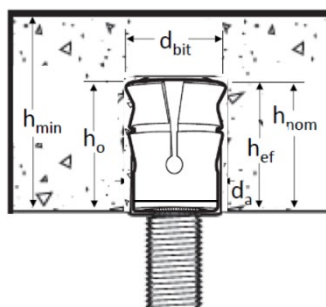
FIGURE 1A—MINI- UNDERCUT+ ANCHOR DETAIL Before (Left Picture) and After (Right Picture) Anchor Setting
