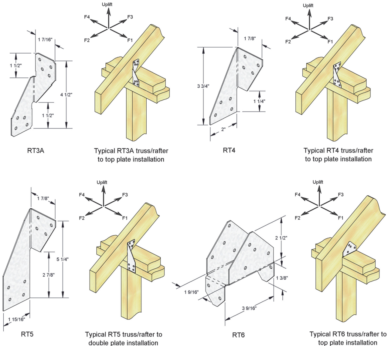
FIGURE 10—RT HURRICANE TIE
