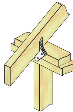
FIGURE 10—RT HURRICANE TIE (Continued)
