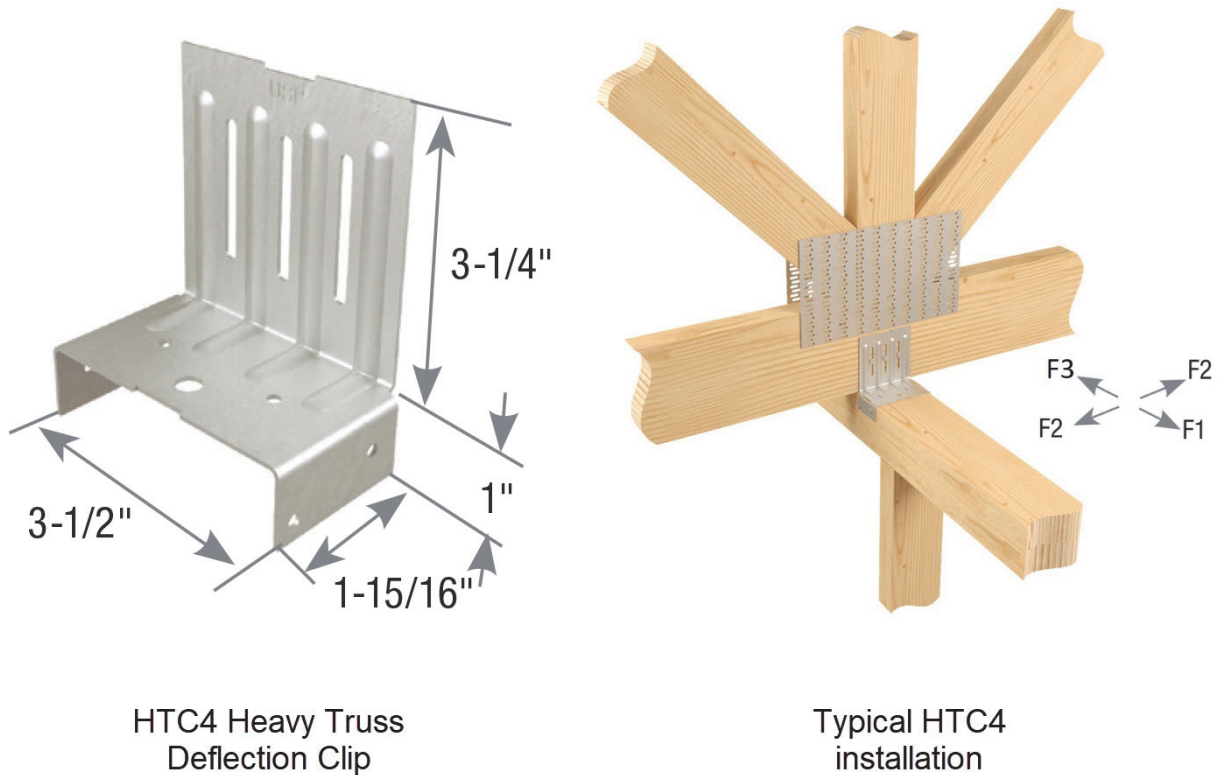
FIGURE 9—HTC HEAVY TRUSS DEFLECTION CLIP
