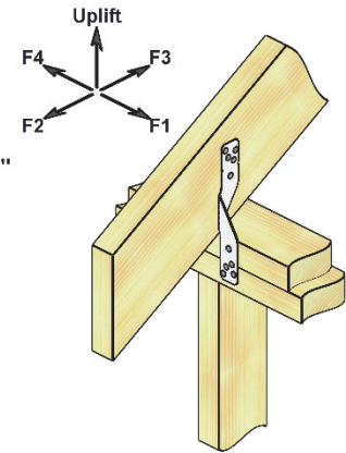
Typical RT8A truss/rafter to double plate installation
