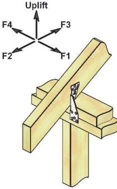
Typical RT7 truss/rafter to double plate installation
