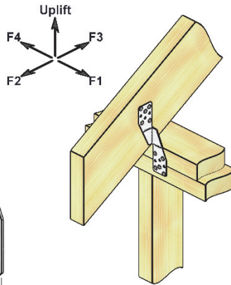
Typical RT7AT truss/rafter to double plate installation
