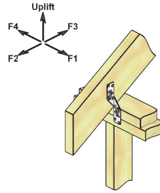
Typical RT7A truss/rafter to double plate installation
