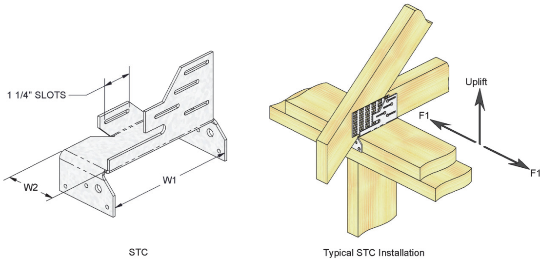
FIGURE 12—STC SCISSOR TRUSS CLIP
