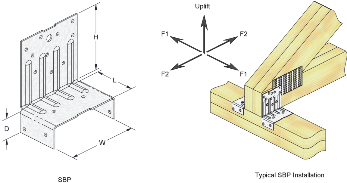
FIGURE 11—SBP SUPPLEMENTARY BEARING PLATE
