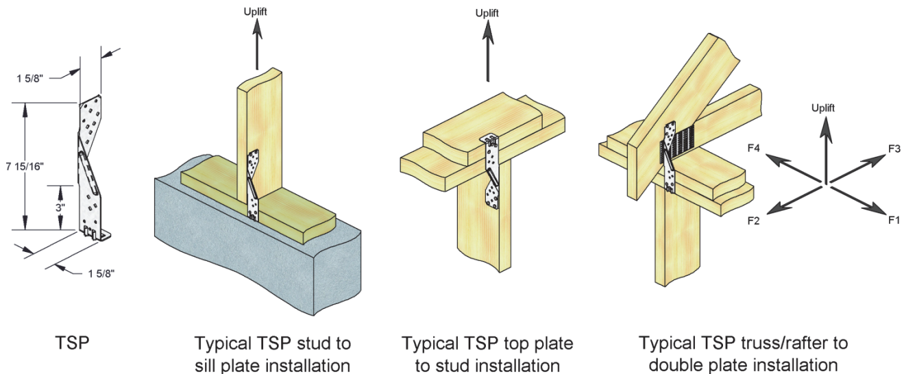
FIGURE 13—TSP STUD PLATE TIE
