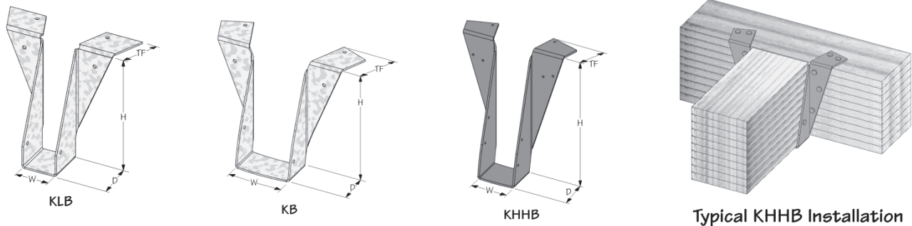
FIGURE 16—KLB, KB, KHHB, KGB, AND KHGB TOP MOUNT HANGERS
