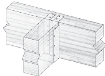
Typical HDO inverted flange installation
