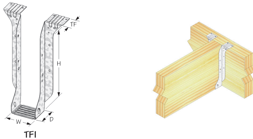
FIGURE 22—TFI TOP MOUNT HANGER AND TYPICAL INSTALLATION
