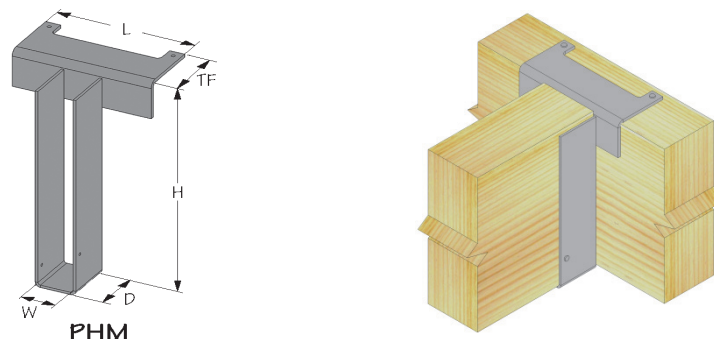
FIGURE 19—PHM TOP FLANGE HANGERS
