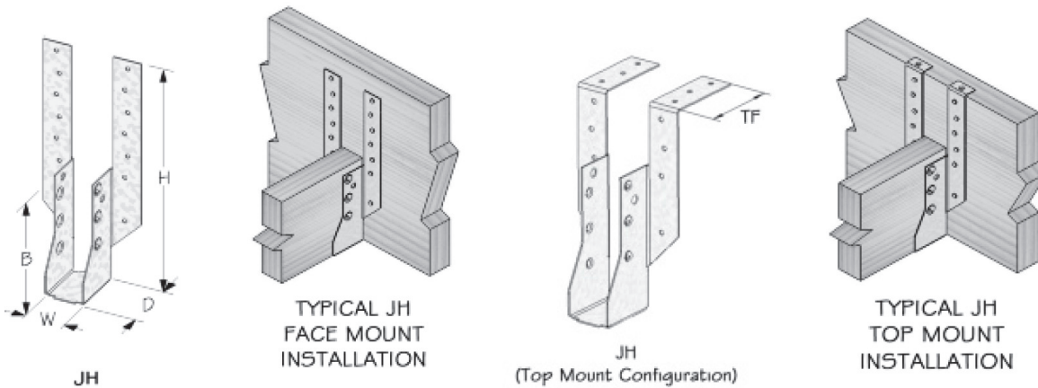
FIGURE 8—DIMENSIONS AND INSTALLATION OF JH JOIST HANGER
