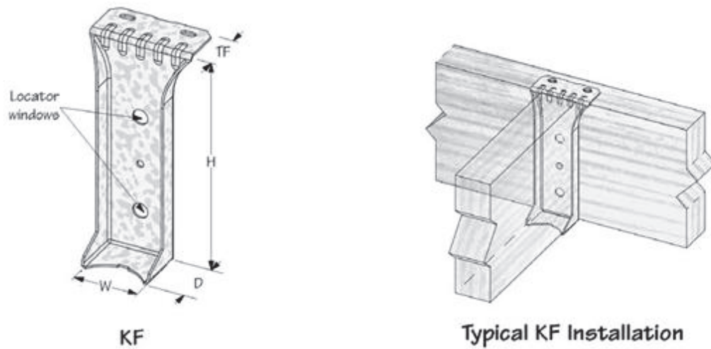
FIGURE 12—KF PANEL HANGER
