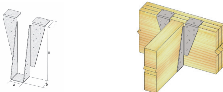
FIGURE 3—HBPH BEAM AND PURLIN HANGER AND TYPICAL INSTALLATION DETAIL
