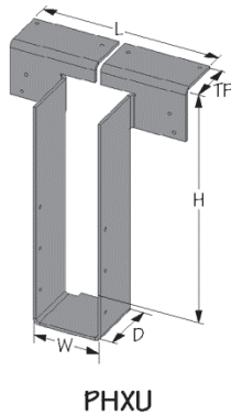
FIGURE 20—DIMENSIONS AND INSTALLATION OF PHXU SERIES HANGERS
