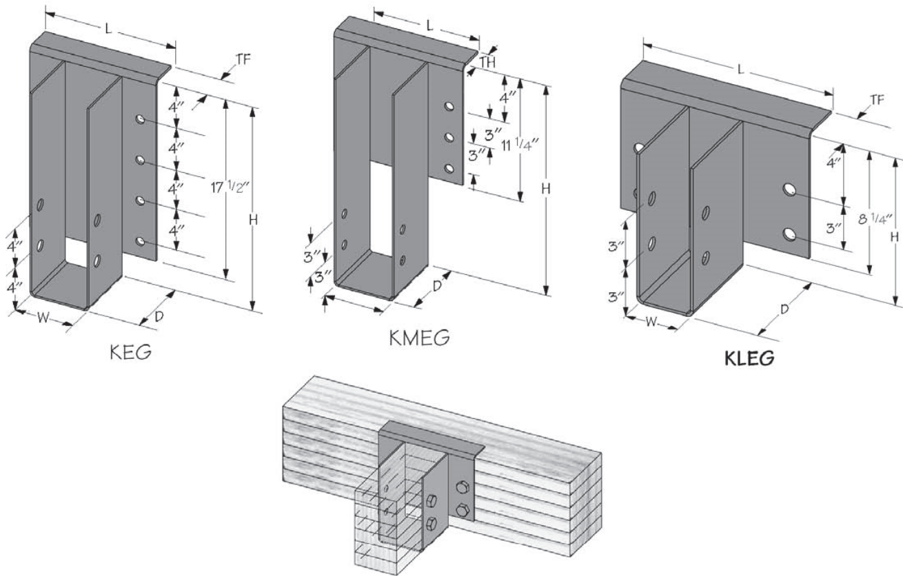
FIGURE 10—KEG, KMEG, & KLEG GLULAM BEAM HANGERS
