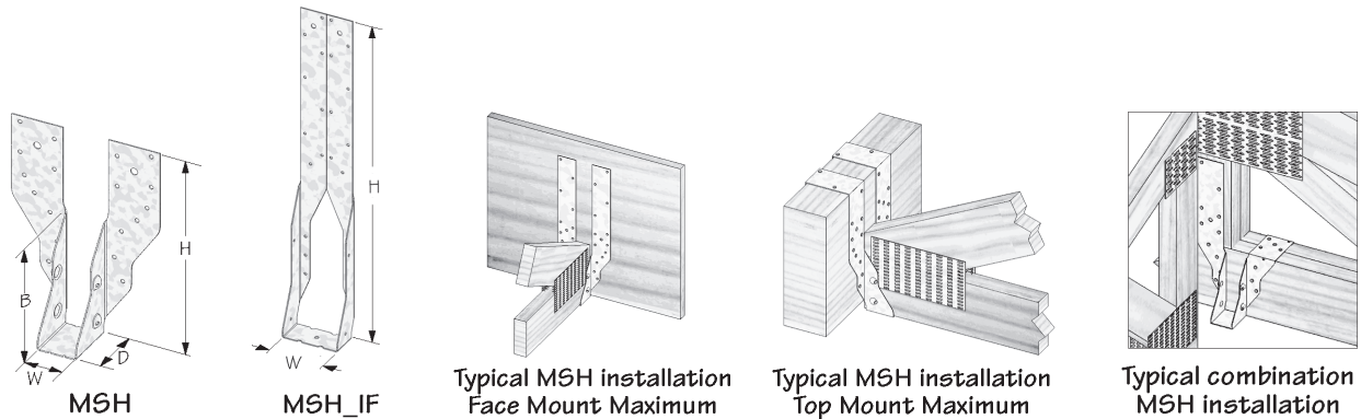
FIGURE 17—MSH STRAP HANGER
