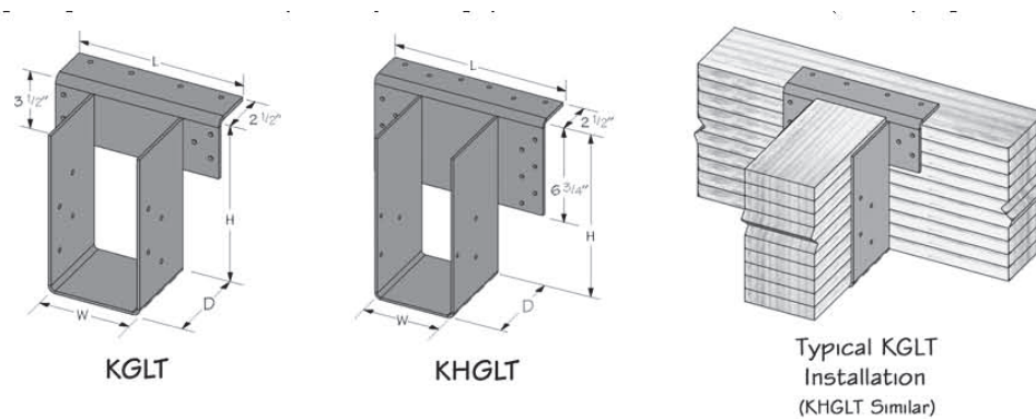
FIGURE 14—KGLT & KHGLT GLULAM HANGERS
