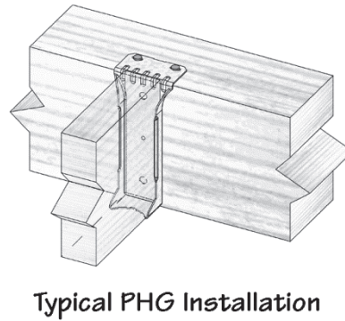
FIGURE 18—PANEL HANGER
