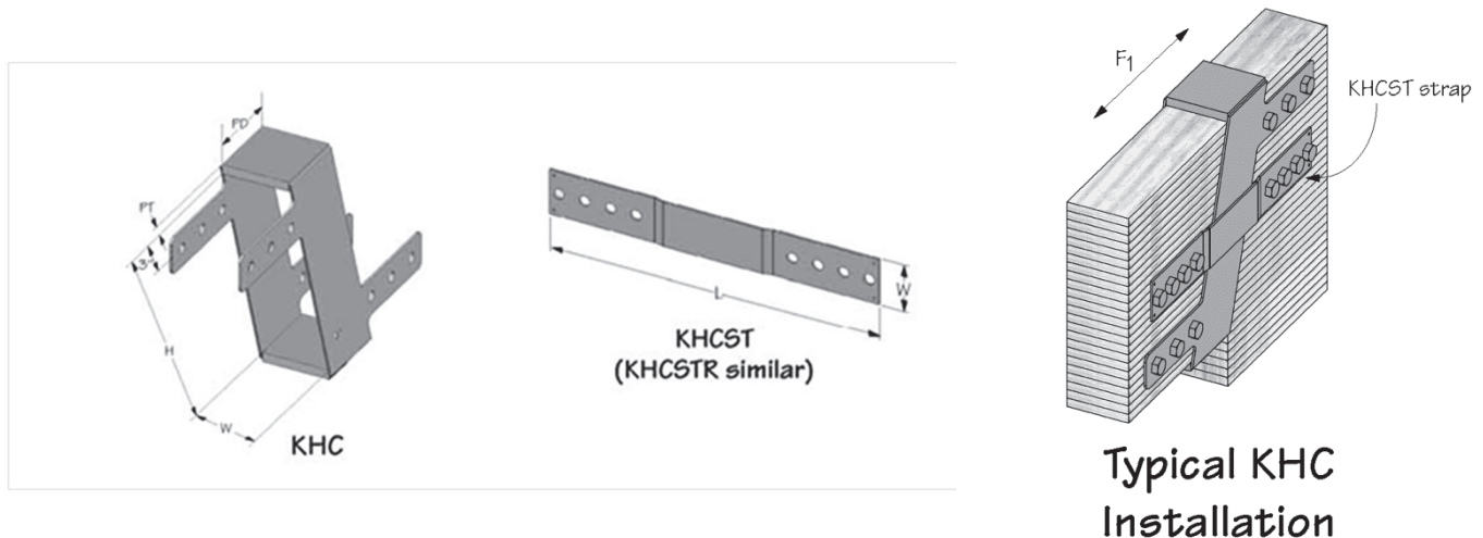
FIGURE 15—KHC HINGE CONNECTOR & KHCST SEISMIC STRAP
