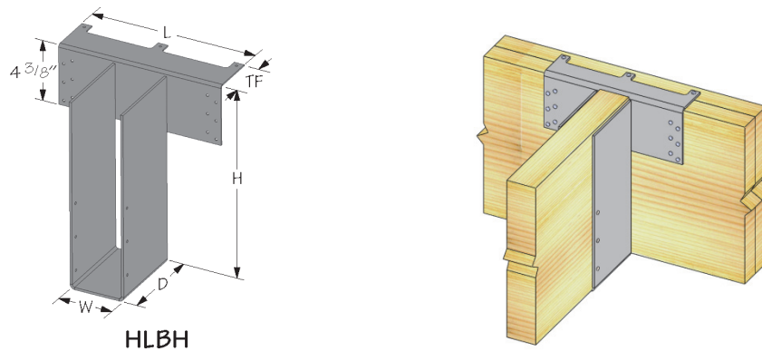
FIGURE 6—HLBH BEAM HANGERS
