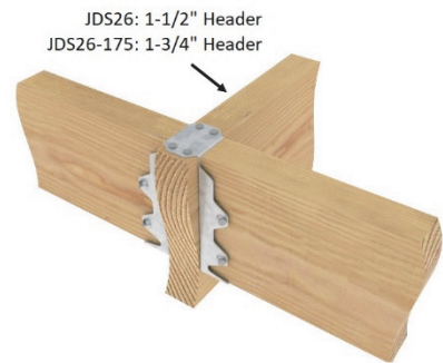
Typical JDS26 / JDS26-175 Installation
