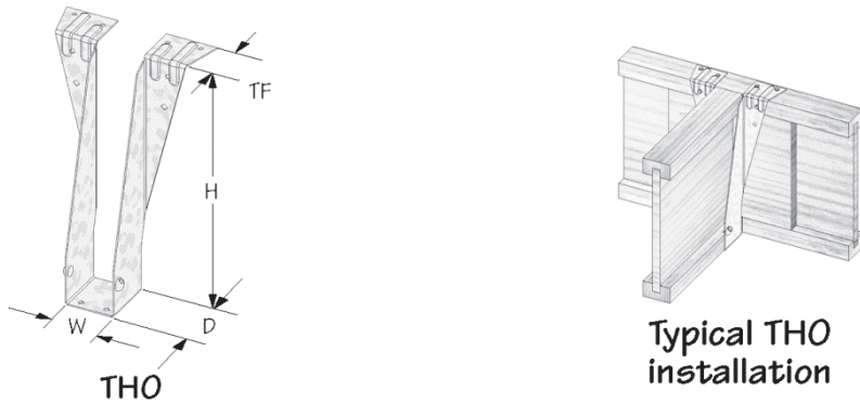
FIGURE 24—THO TOP MOUNT HANGER
