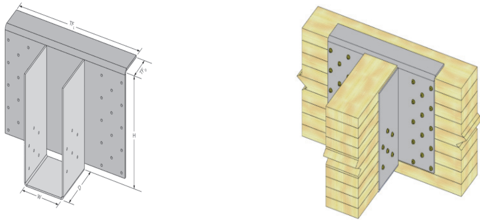
FIGURE 11—KEGQ TOP MOUNT GIRDER HANGER AND TYPICAL INSTALLATION DETAIL
