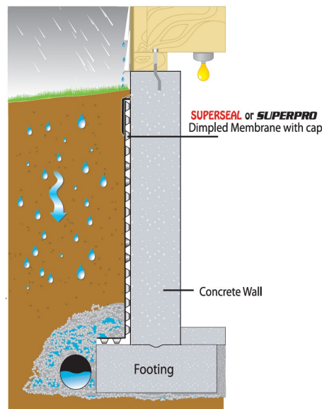
FIGURE 1—TYPICAL MEMBRANE INSTALLATION DETAIL
