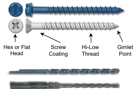
UltraCon+ Bits FIGURE 2—ULTRACON+ SCREW ANCHOR AND DRILL BITS
