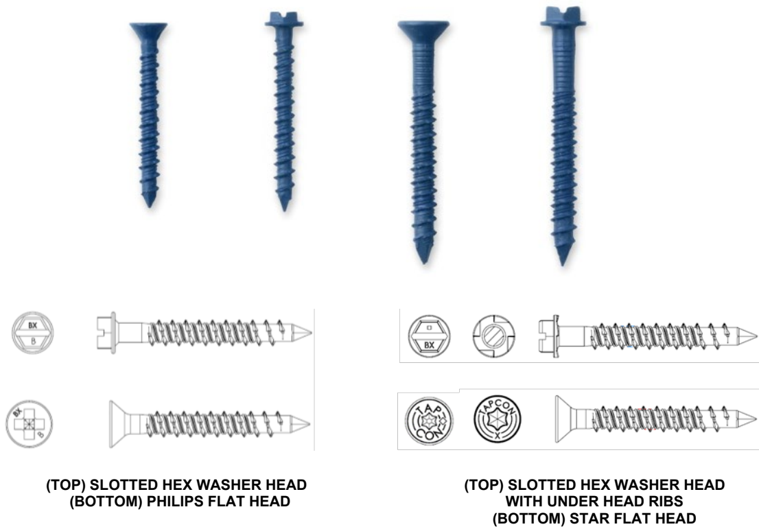
FIGURE 1—TAPCON® SCREW ANCHOR WITH ADVANCED THREADFORM TECHNOLOGY (BLUE CLIMASEAL® COATING SHOWN)
