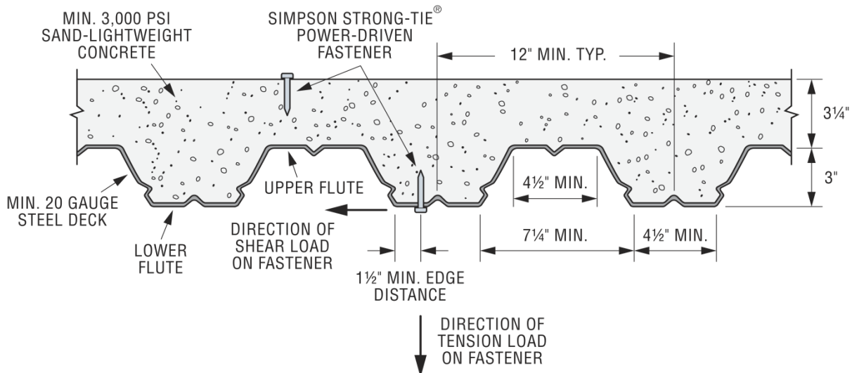
FIGURE 8—INSTALLATION IN 3 1/4-INCH CONCRETE FILL OVER 3-INCH-DEEP STEEL DECK
