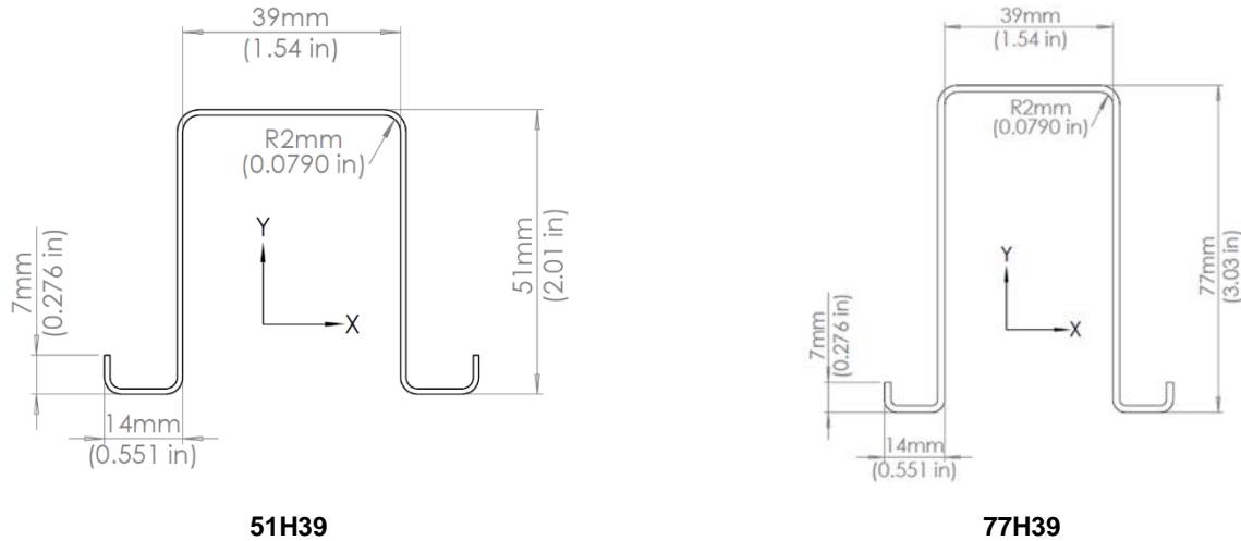
FIGURE 1—HAT SECTIONS
