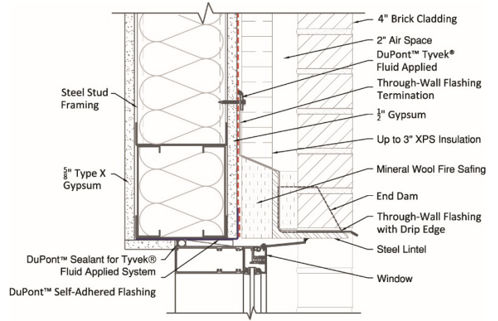
NFPA 285 Window Head Detail Option #4
