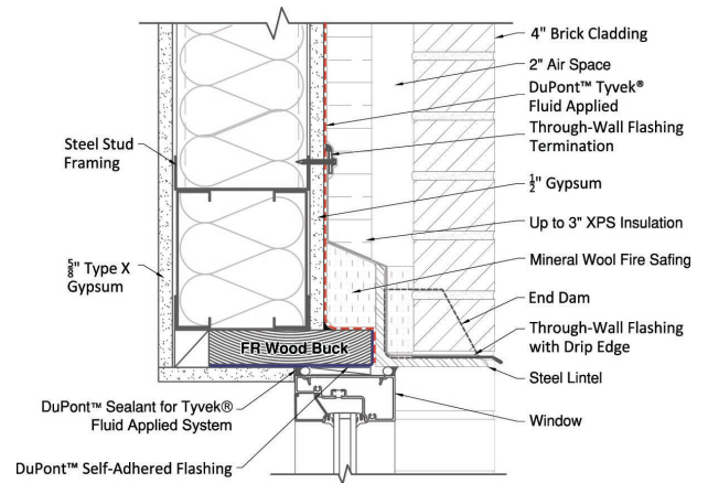
NFPA 285 Window Head Detail Option #6
