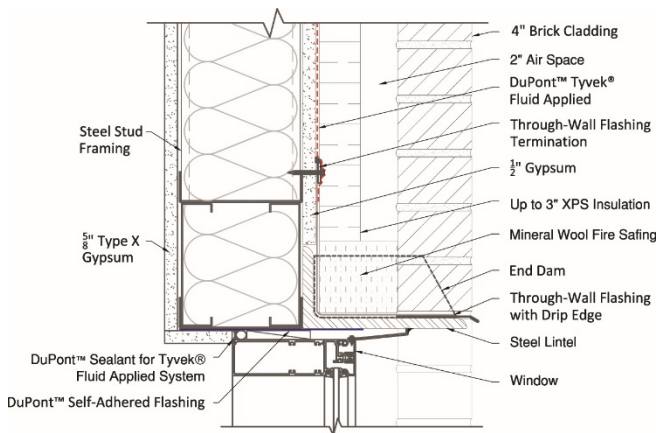
NFPA 285 Window Head Detail Option #1
