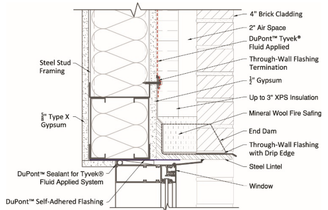
NFPA 285 Window Head Detail Option #2
