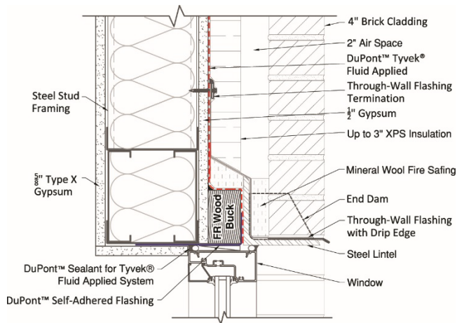
NFPA 285 Window Head Detail Option #5
