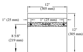
FIGURE 1—SHINGLE PROFILES AND FASTENER PATTERNS (Continued)
