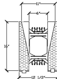
CROSS SECTION OF 6" TAPERED TOP FORM
