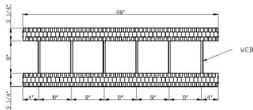
PLAN OF STRAIGHT BLOCK
