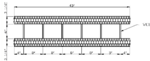
PLAN OF STRAIGHT BLOCK
