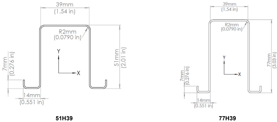
FIGURE 1—HAT SECTIONS
