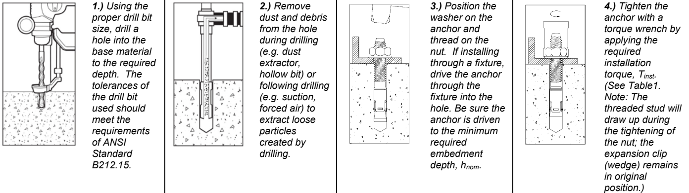
FIGURE 2—POWER-STUD+ SD1 INSTALLATION INSTRUCTIONS
