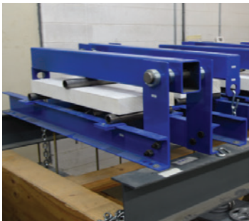
Flexural Creep
