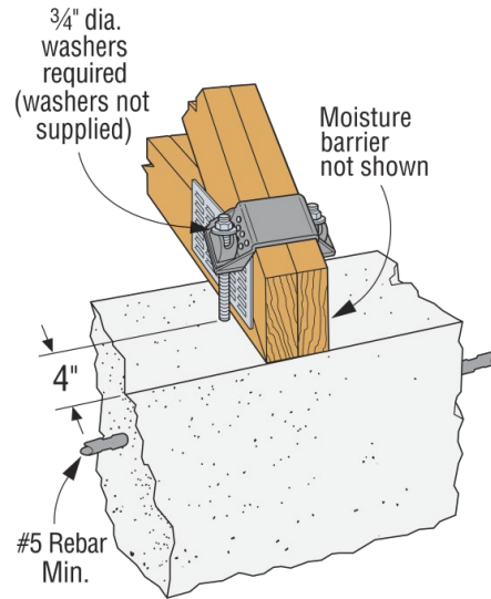
Typical HGT-2 Installation to Concrete Construction
