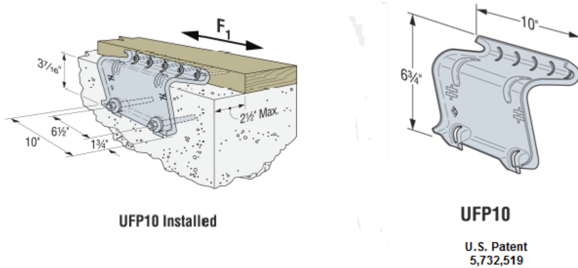
FIGURE 1—UFP UNIVERSAL FOUNDATION PLATE
