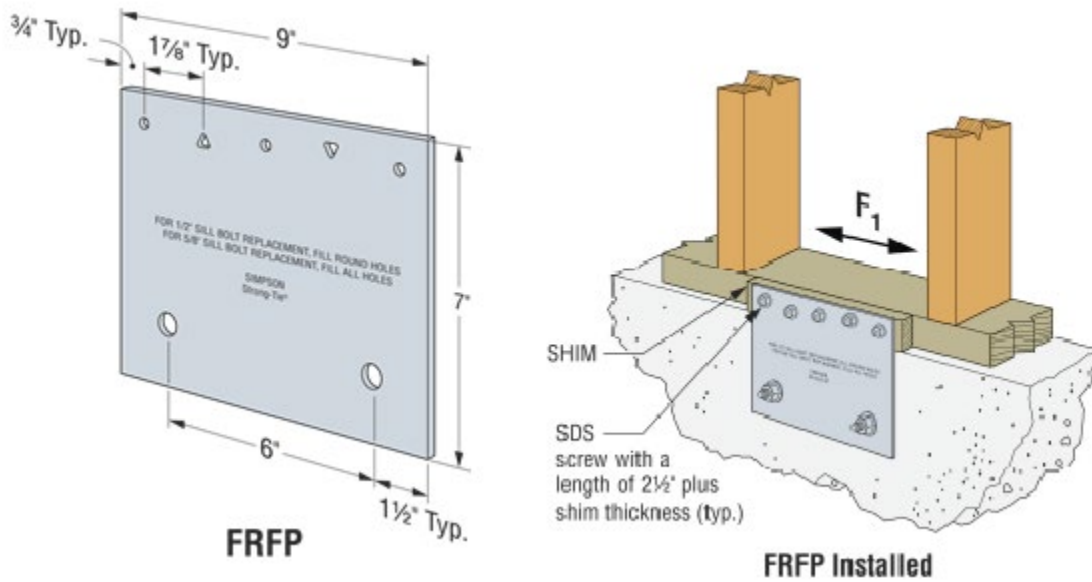
FIGURE 8—FRFP FLAT RETROFIT FOUNDATION PLATE
